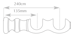
Double 40/48 Bracket
